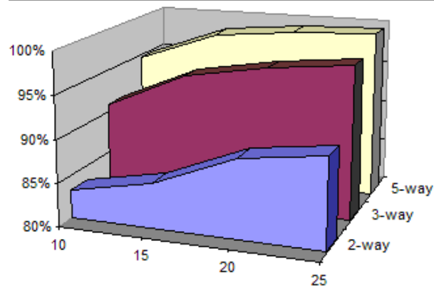
Figure 23. Percent coverage of t -way combinations for v=8 .
